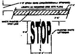
STOP BAR AND LEGEND NO SCALE
