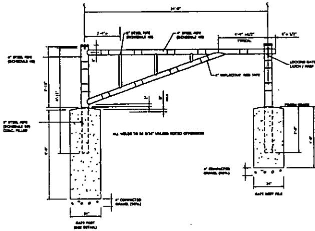
SWING GATE NO SCALE
